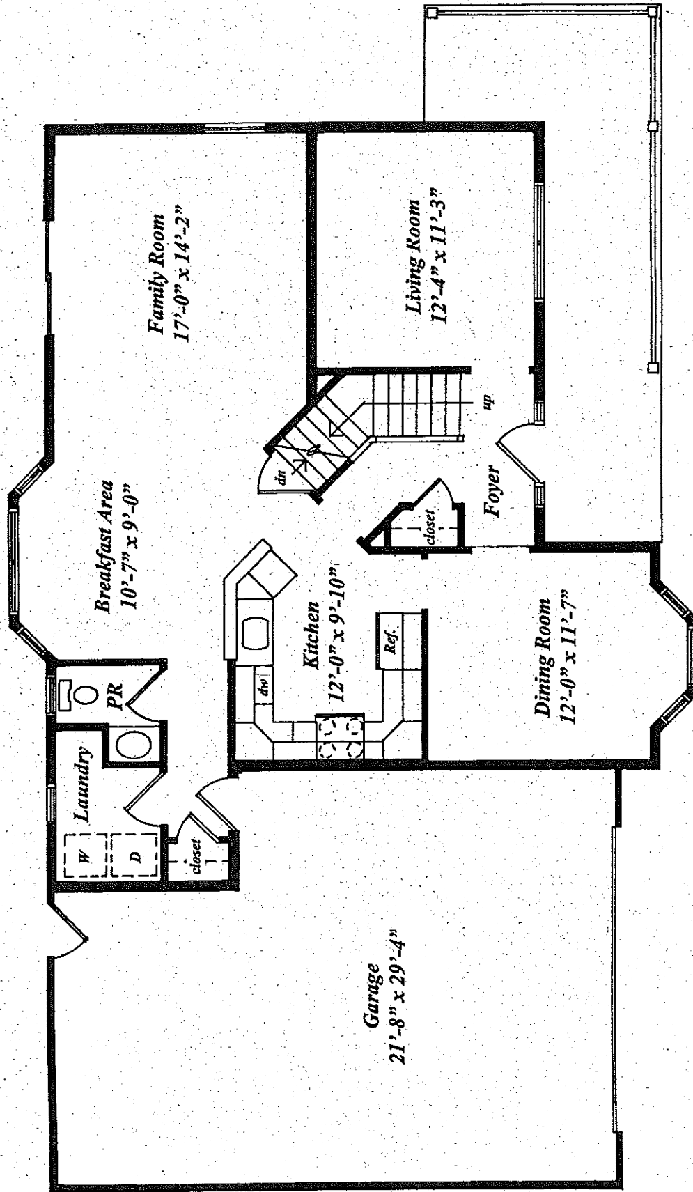
First Floor Plan 40'-4" x 34'-0"
